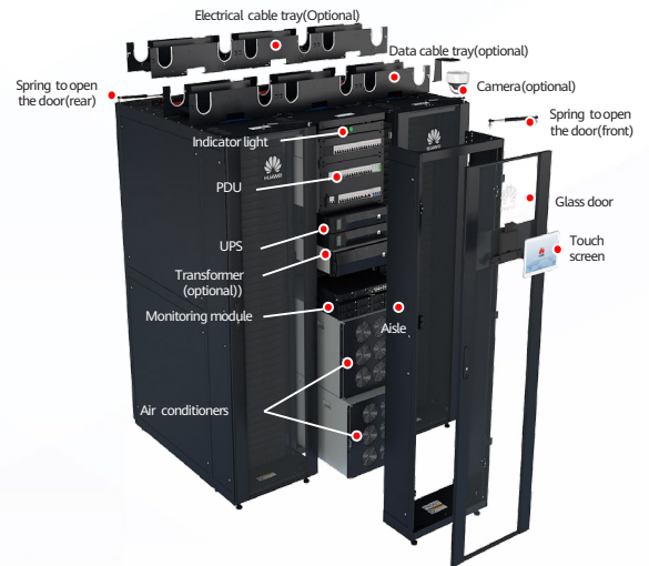
FusionModule800 Architecture
